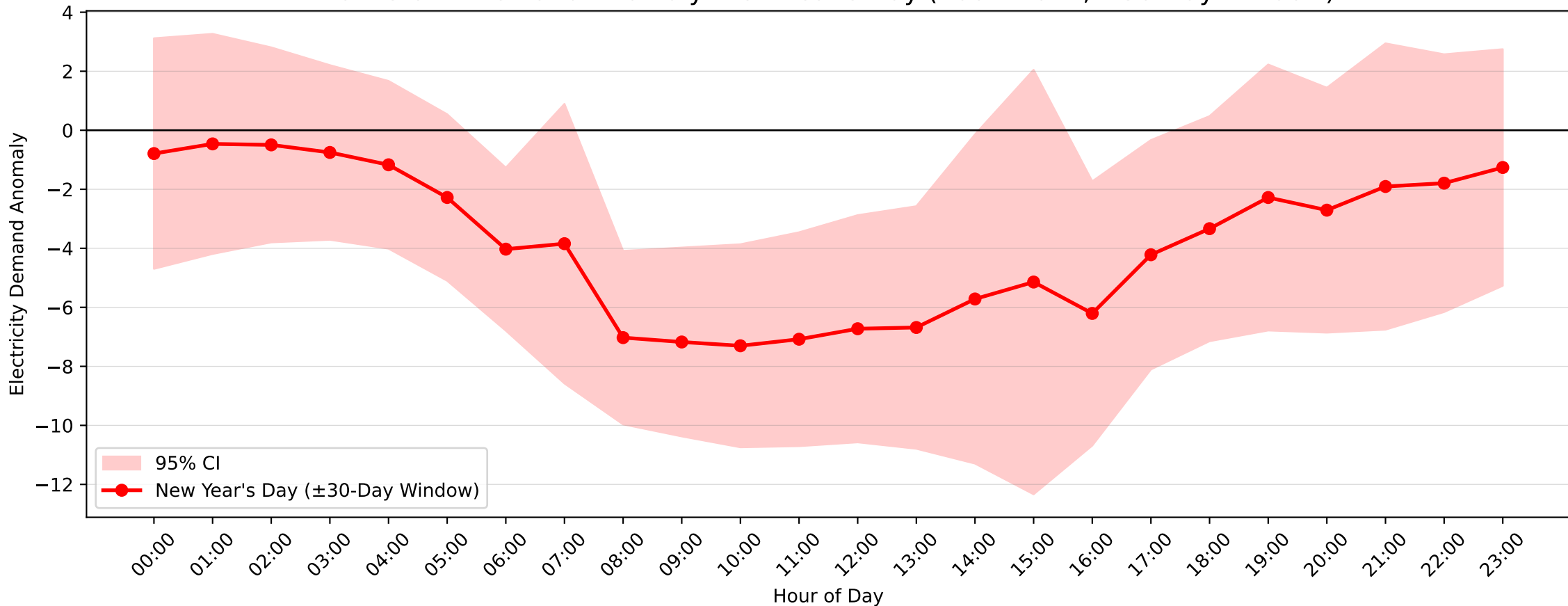
Bankstown Demand Anomaly: New Year's Day (2004-2017, \pm 30 -Day Window)
